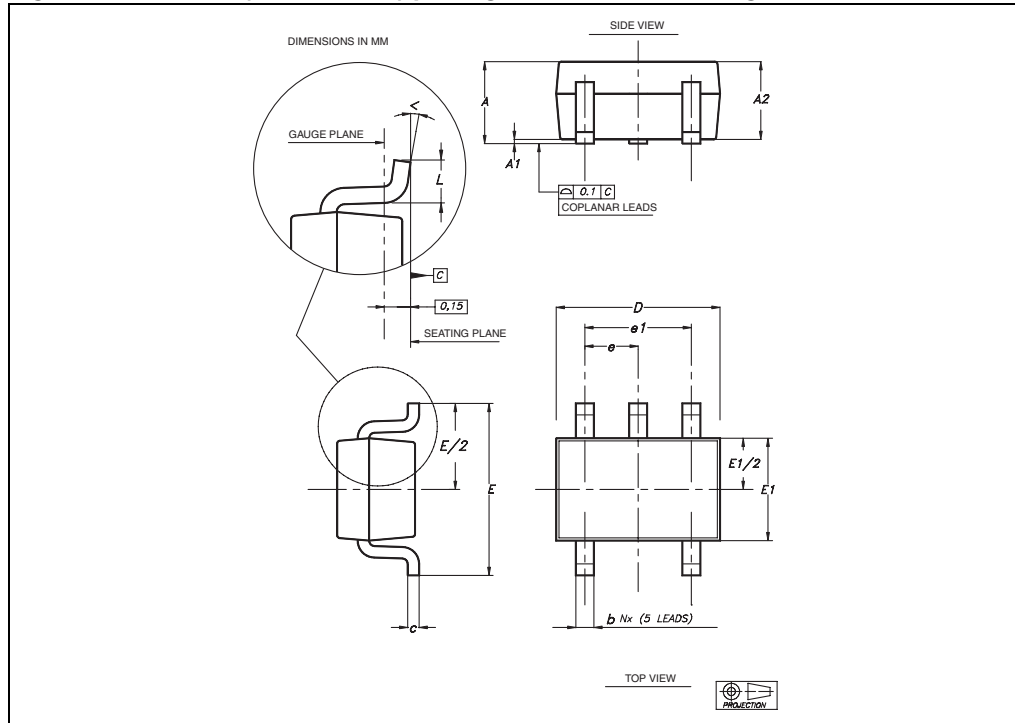
Figure 23. SC70-5 (or SOT323-5) package mechanical drawing
