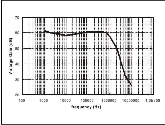
Figure 17. Frequency response of the global preamplifier chain
