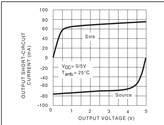
Figure 5. Output short circuit current vs. output voltage
