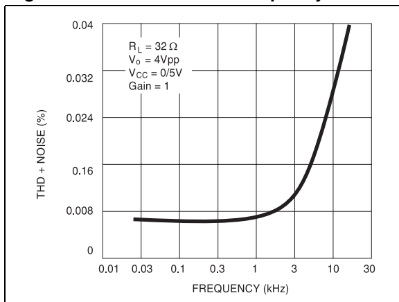
Figure 11. THD + noise vs. frequency
