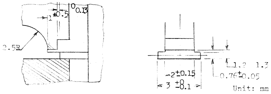
Recommended Housing Tab Entry Design Drawing
