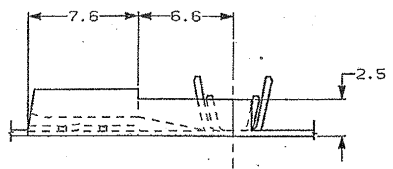
SECTION A-A SECTION B-B
