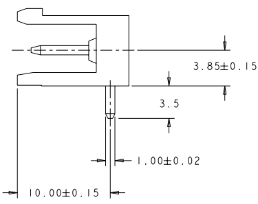
1776158-2 AS SHOWN
