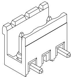
1776158-2 AS SHOWN
