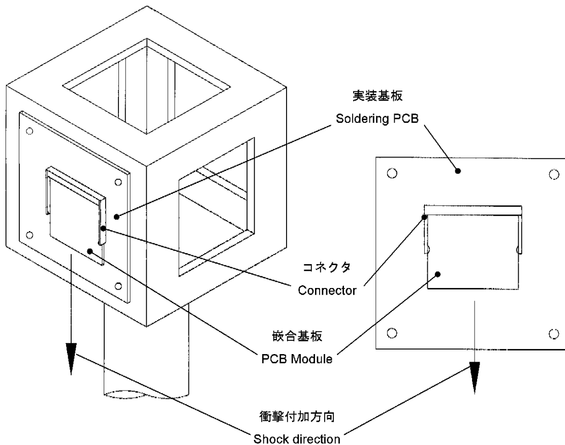
Fig. 3-2 衝撃試験 (耐久試験) Fig3-2 Physical Shock (Durable tetst)
