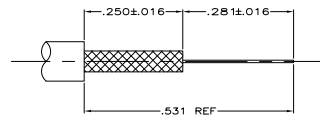
VIEW D RECOMMENDED STRIP LENGTH
