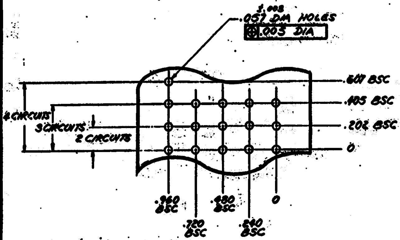
P.C. BOARD LAYOUT FOR 5, 6, 9, 12, AND 15 CIRCUIT PANEL MOUNT HOUSINGS
