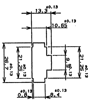
推奨パネル開孔寸法 (RECOMMENDED PANEL OPENING DIMENSION) FIG 1
