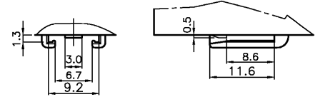
CLIP HOLE DETAIL
