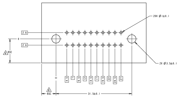
P.C. BOARD LAYOUT RECOMMENDED THICKNESS: 1.6mm TOLERANCE: ±0.1 SCALE 4:1
