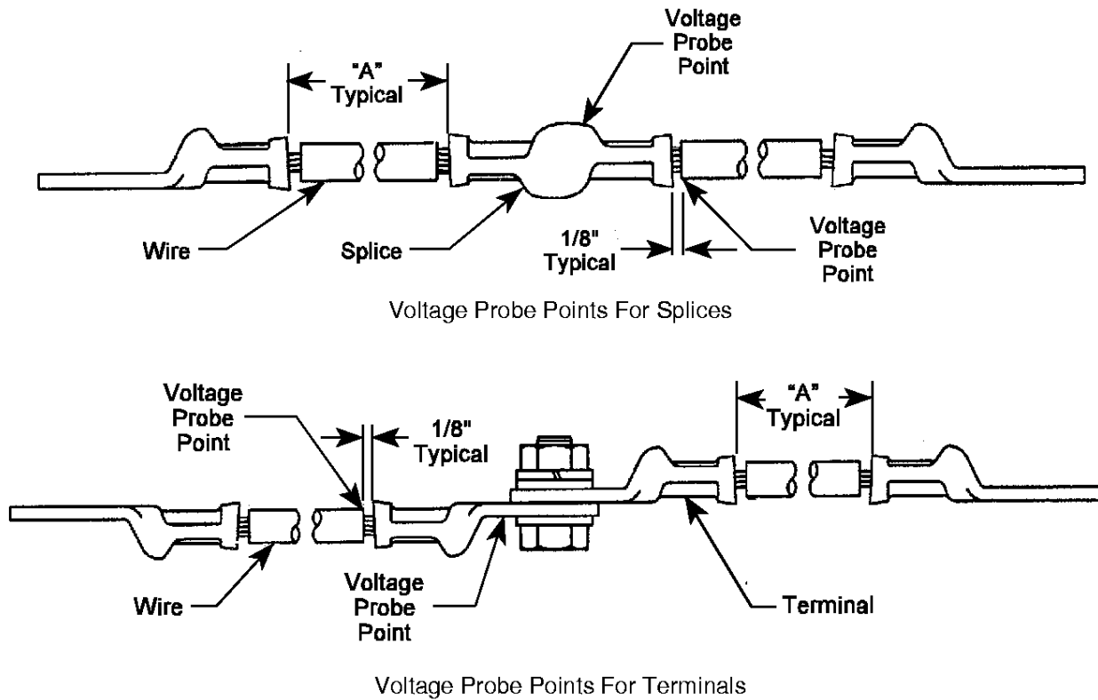
Figure 4 Voltage Probe Points
