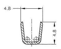
断面 "A"- "A" SECT "A"- "A"
