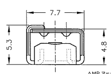
断面 "B"- "B" SECT "B"- "B"
