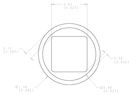
△ SOLDER TERMINATION AREA SCALE 40:1 RECOMMENDED PRINTED CIRCUIT SOLDER HOLE COMPLIANT PRESS FIT DRILLED HOLE: \varnothing 1.15 [0.0453] \pm .013 [0.0005] COPPER PLATE: .025 (.0010) MIN (PER SIDE) TIN PLATE: .0005 [0.00020] MIN. (PER SURFACE)
