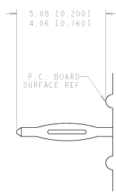
6. COMPLIANT PIN DETAIL SCALE 10:1 INSERTION/EXTRACTION FORCES MAXIMUM PUSH IN: 133.3N (30 LBS) PER PIN MINIMUM PUSH OUT: 44.4N (10 LBS) PER PIN
