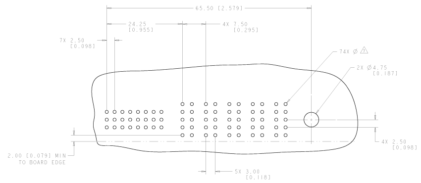
PRINTED CIRCUIT LAYOUT
