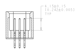
SECTION Z-Z GENDER CHANGER REMOVED FOR CLARITY
