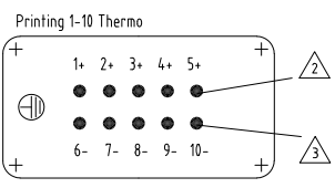
Contact arrangement view from termination side
