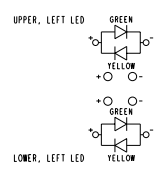
6368116-3 LED SCHEMATIC
