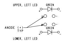
6368116-1, -2 LED SCHEMATIC
