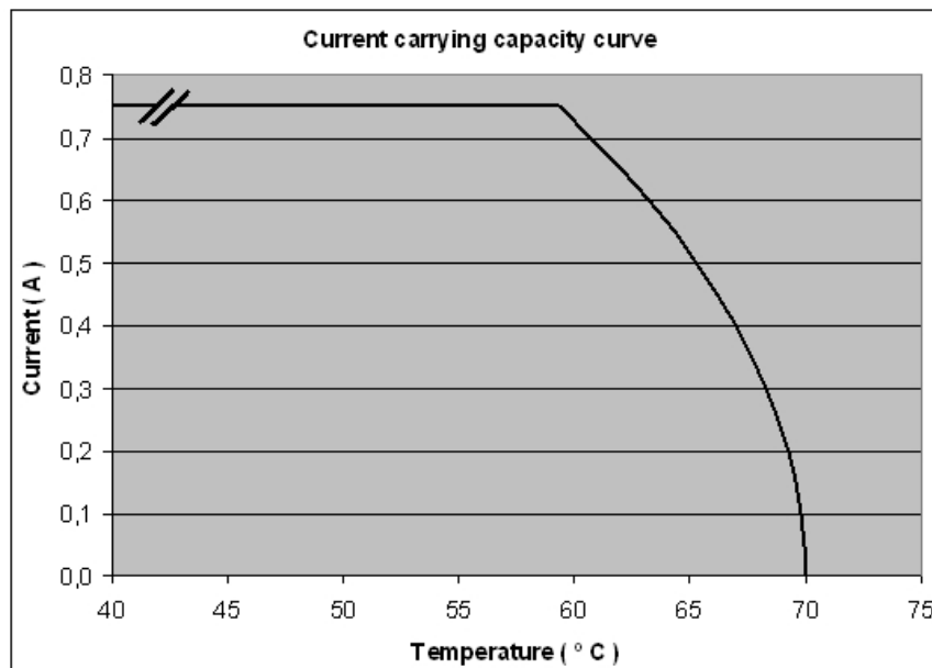
Figure 5 Current-carrying capacity
