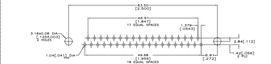
RECOMMENDED P.C. BOARD MOUNTING DIMENSIONS P.C. BOARD THICKNESS: 1.57[0.062]
