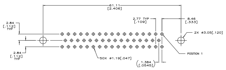
RECOMMENDED PC BOARD MOUNTING DIMENSIONS
