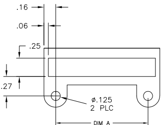
RECOMMENDED PANEL LAYOUT
