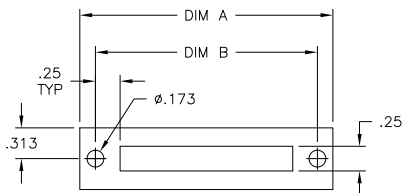
RECOMMENDED BOARD LAYOUT
