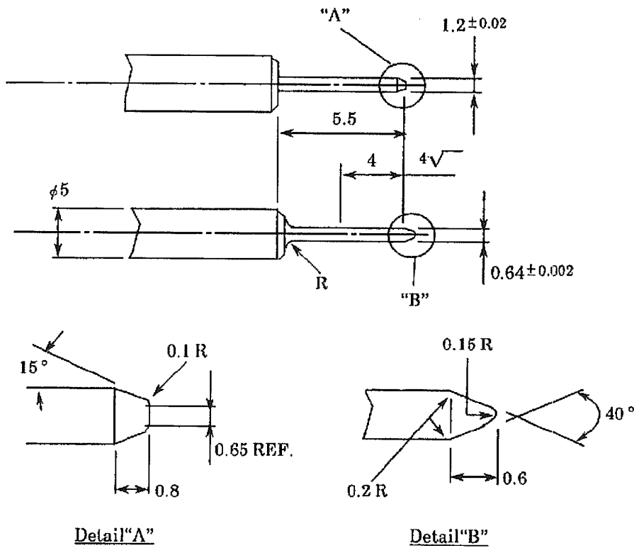
Fig. 10 Contact Insertion / Extraction Force Measuring Gage Design
