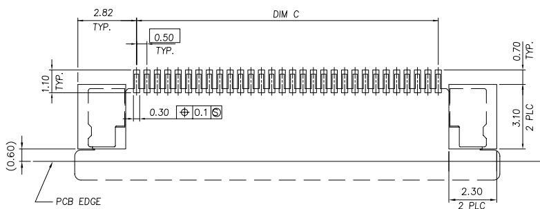
RECOMMENDED PCB DIMENSIONS DIAGRAM TOLERANCE: ±0.05
