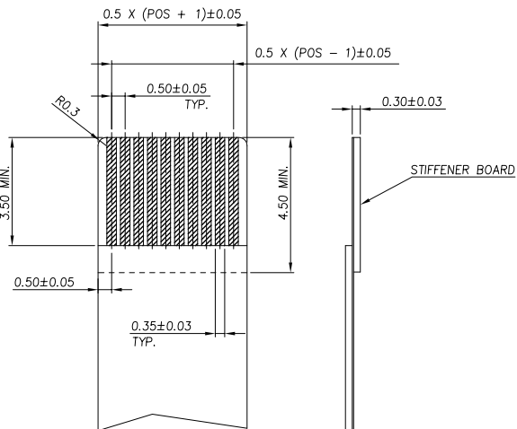
RECOMMENDED FPC DIMENSIONS DIAGRAM
