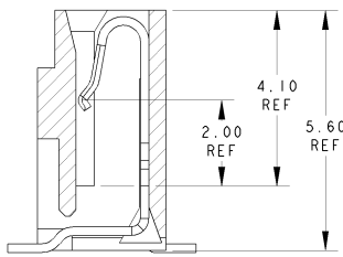
SECTION A-A (FOR EVEN POSITION CONTACTS) SCALE 10:1
