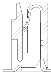
SECTION B-B (FOR ODD POSITION CONTACTS) SCALE 10:1
