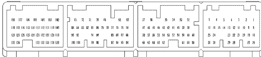
Fig.12 135 Position Circuit Layout
