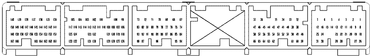
Fig.13 167 Position Circuit Layout
