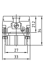
Contact arrangement view from termination side
