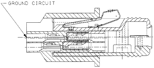
SECT "A"-"A" (SCALE 2-1)
