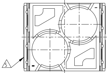
CONTACT ARRANGEMENT VIEW FROM TERMINATION SIDE
