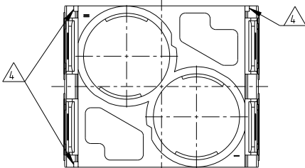
CONTACT ARRANGEMENT VIEW FROM CONNECTING SIDE
