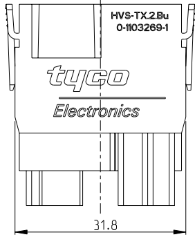
CONTACT ARRANGEMENT VIEW FROM TERMINATION SIDE
