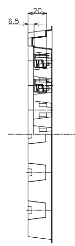
SECTION B-B
