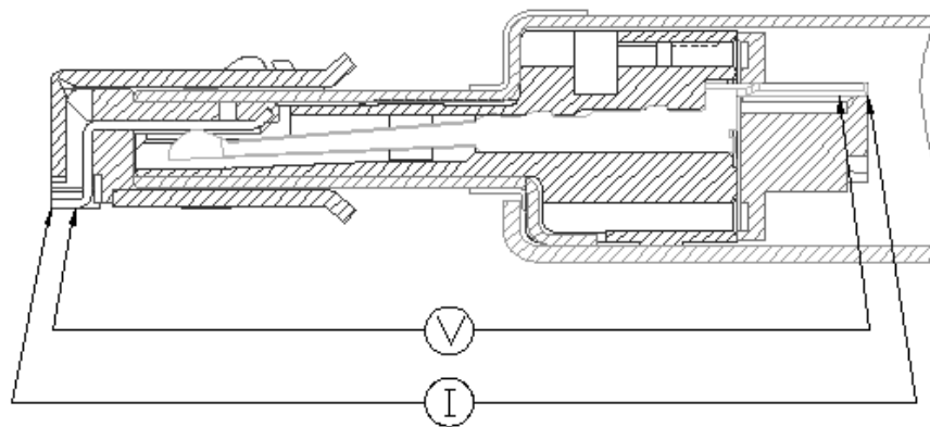
Fig.2 Measuring method of contact resistance
