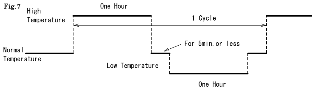
Thermostatic chamber temperature is set at 125°C as the high temperature and -40°C as the low temperature
