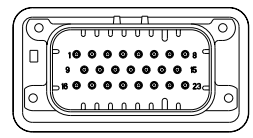
776228-4 & 1-776228-4 KEY LOCATION SCALE 2:1
