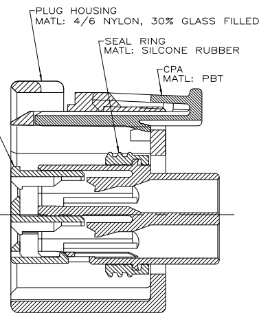
SECTION Z-Z SCALE 4:1
