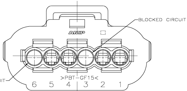
VIEW B-B
