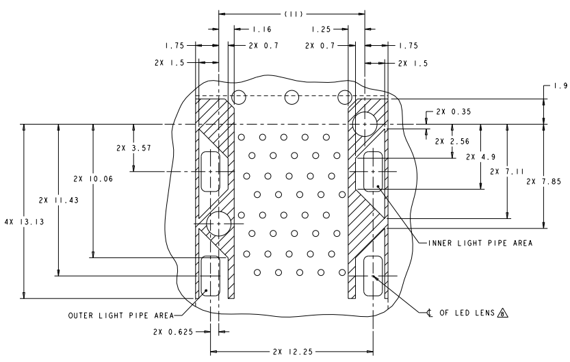
DETAIL G CONNECTOR HOUSING KEEPOUT ZONE SCALE 10:1
