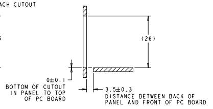
SECTION U-U
