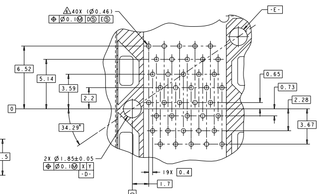
DETAIL F 4X INDIVIDUALLY SCALE 10:1
