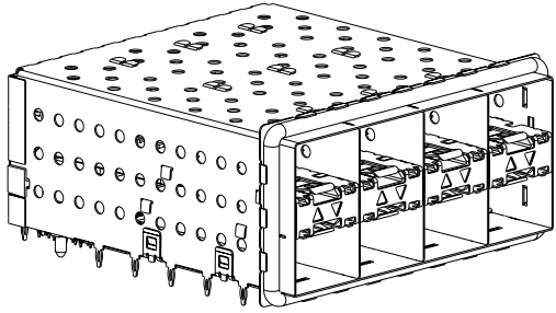
2007399-2 AND 2007399-6 SCALE 3:1
