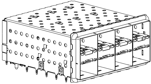
2007399-4 AND 2007399-8 SCALE 3:1
