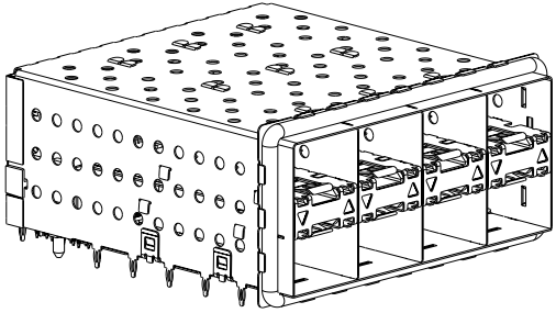
2007399-3 AND 2007399-7 SCALE 3:1
