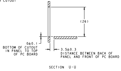
SECTION U-U
