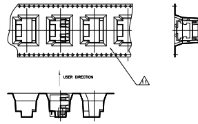
DETAIL B TAPE REEL PACKAGE SCALE 2:1
