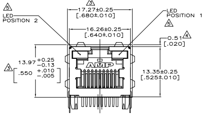
VIEW OF 3-406549-8
