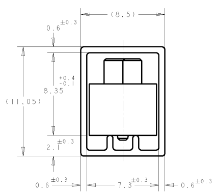
DETAIL "A" (SCALE 5-1)
