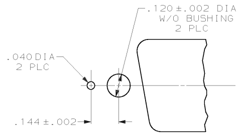
PANEL CUTOUT DETAIL NTS
