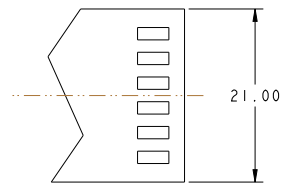
RECOMMENDED PCB LAYOUT FOR 1971567-3 (±0.10mm) SCALE 3:1
