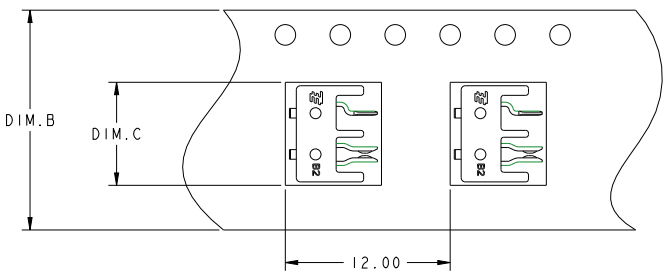
TO BE PACKAGED AS SHOWN (±0.10mm) SCALE 5:1
