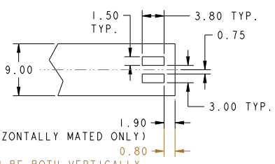
(TYPE 1: HORIZONTALLY MATED ONLY) (TYPE 2: CAN BE BOTH VERTICALLY AND HORIZONTALLY MATED) RECOMMENDED PCB LAYOUT FOR 1971567-1 (±0.10mm) SCALE 3:1
