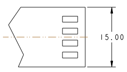
RECOMMENDED PCB LAYOUT FOR 1971567-2 (±0.10mm) SCALE 3:1
