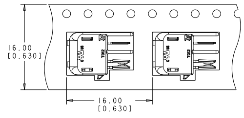
TO BE PACKAGED AS SHOWN SCALE 4:1
