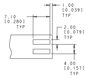
RECOMMENDED PCB LAYOUT FOR 2058703-1 & 1-2058703-1
