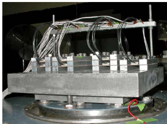
Figure 4 Vibration and Mechanical Shock Mounting Fixture
