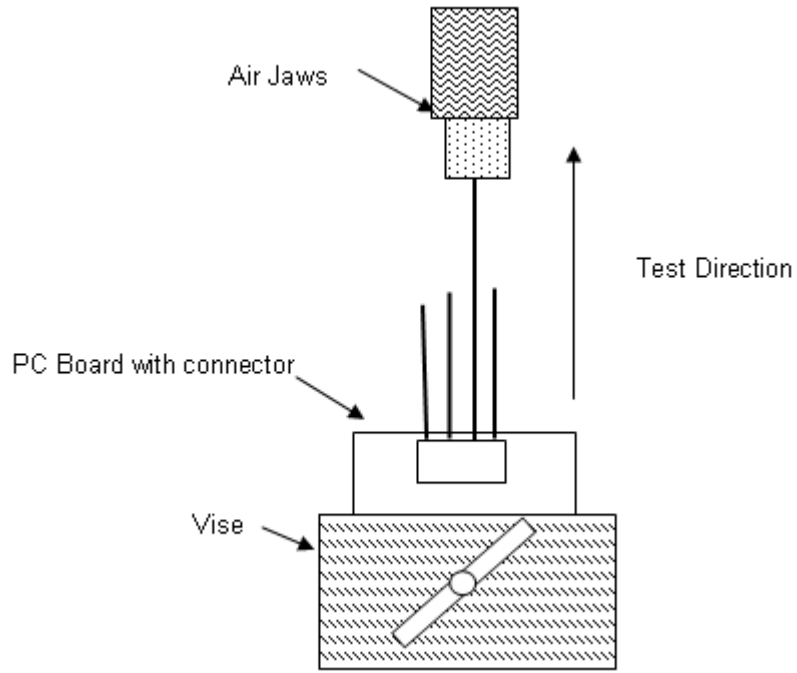
Figure 6 Termination Tensile Strength, Parallel
