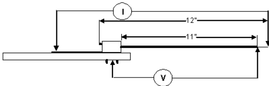
Figure 3 LLCR Measurement Points
