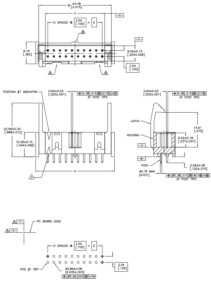
RECOMMENDED PC BOARD LAYOUT (VIEWED FROM CONNECTOR SIDE)
