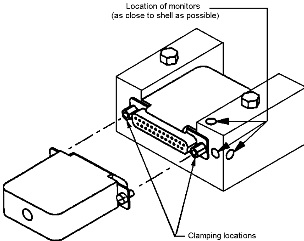
Figure 4 Vibration and Physical Shock Mounting and Clamping Locations
