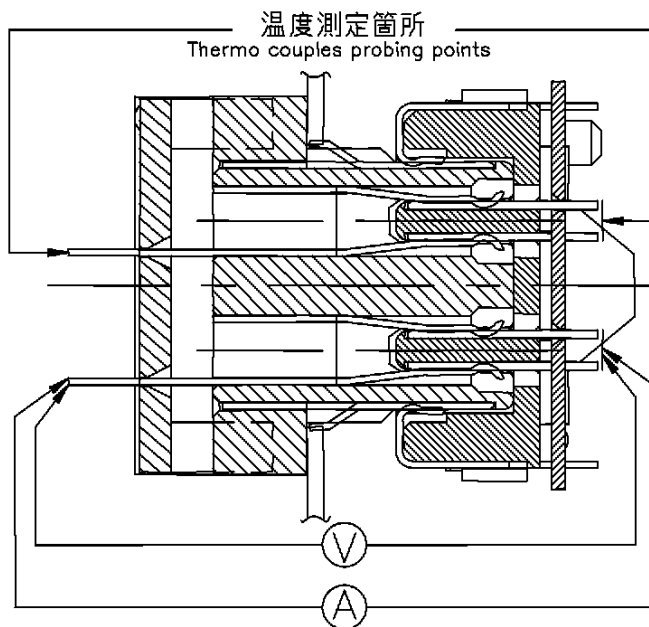
Fig. 3 ロレベル総合抵抗測定点 Fig3 Termination Resistance Measuring points
