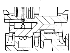
SECTION A-A (BEFORE CRIMPING) SCALE 5:1
