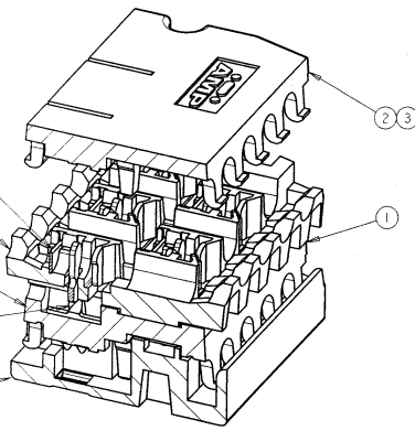
PERSPECTIVE OF SECTION A-A (BEFORE CRIMPING) SCALE 5:1
