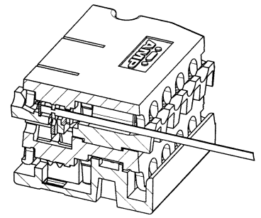
PERSPECTIVE OF SECTION A-A (AFTER CRIMPING) SCALE 5:1
