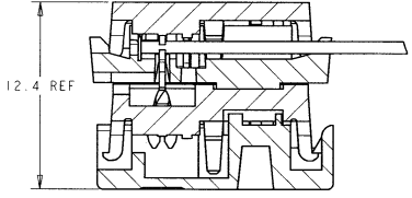
SECTION A-A (AFTER CRIMPING) SCALE 5:1
