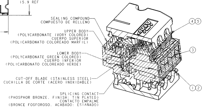
PERSPECTIVE OF SECTION A-A (BEFORE CRIMPING) SCALE 5:1
