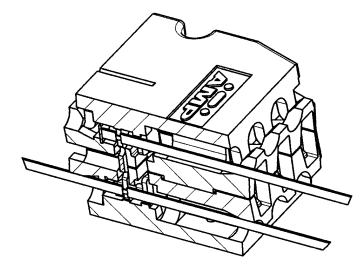
PERSPECTIVE OF SECTION A-A (AFTER CRIMPING) SCALE 5:1
