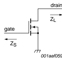
Fig 3. Definition of transistor impedance
