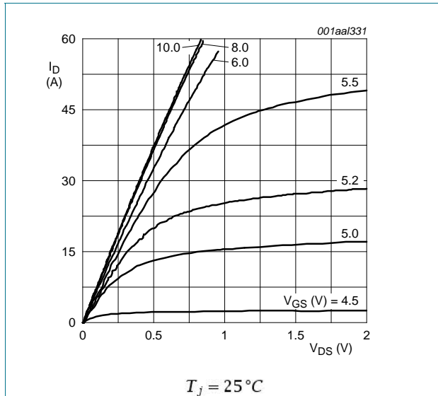
Fig 9. Output characteristics: drain current as a function of drain-source voltage; typical values
