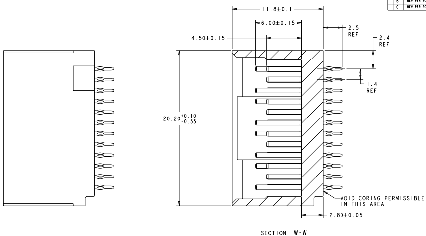
SECTION W-W
